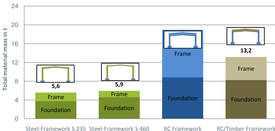
Figure 9: Quantities for the structural systems: frames and foundations, in t
