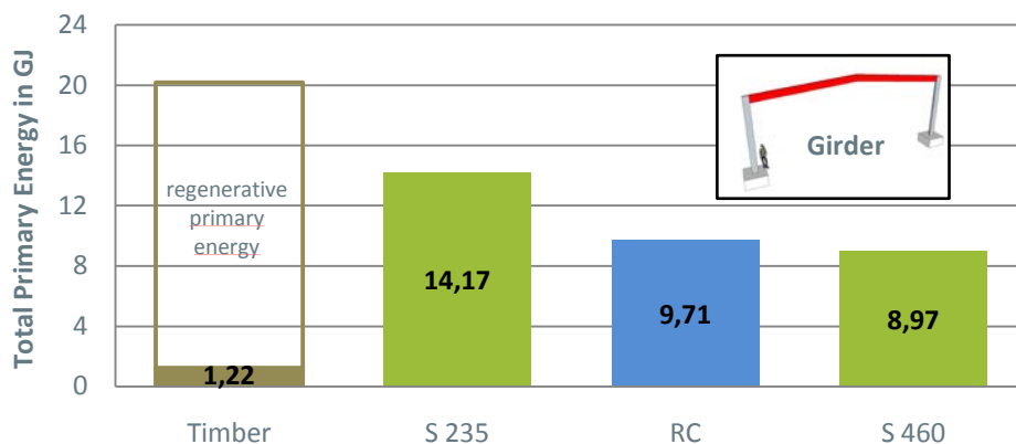
Figure 21: Total Primary Energy or the Product Stage (A1-A3) summed up with Benefits & Loads (D) from recycling (steel), incineration (timber) or rubble processing (concrete) for one girder, in GJ
