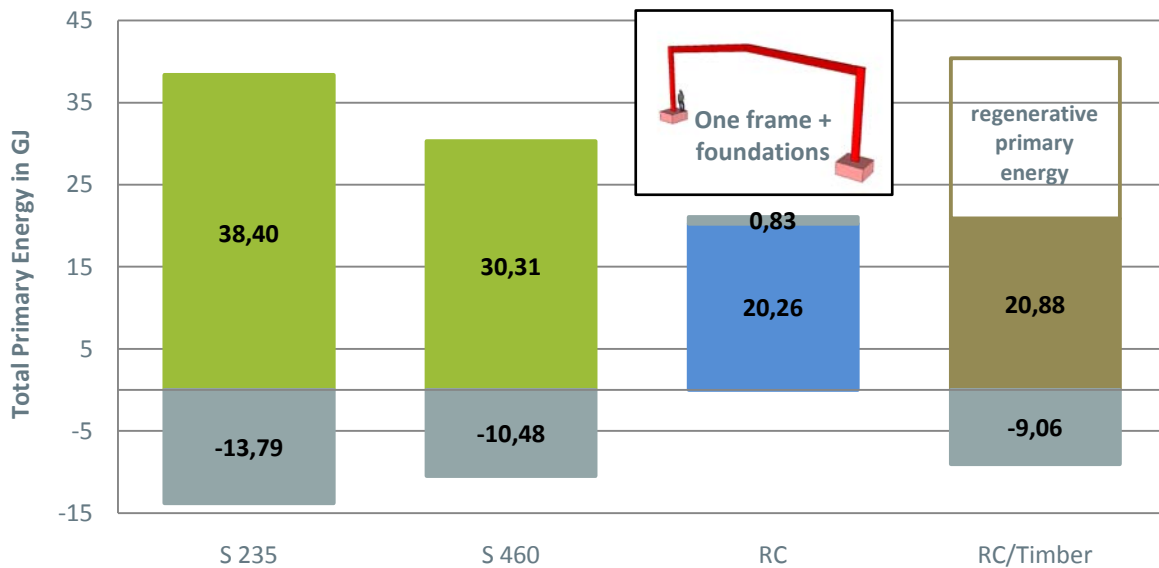
Figure 12: Total Primary Energy for the Product Stage (A1-A3) and separately Benefits & Loads (D, grey) from recycling (steel), incineration (timber) or rubble processing (concrete) for one frame with foundations, in GJ
