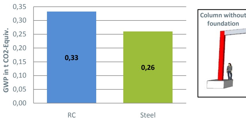
Figure 17: Global Warming Potential for the Product Stage (A1-A3) summed up with Benefits & Loads (D) from recycling (steel), incineration (timber) or rubble processing (concrete) for one column without foundation, in t CO2-Equivalent
