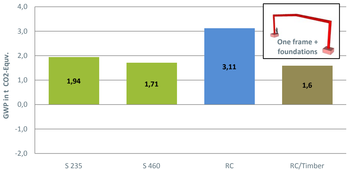
Figure 11: Global Warming Potential for the Product Stage (A1-A3) summed up with Benefits & Loads (D) from recycling (steel), incineration (timber) or rubble processing (concrete) for one frame with foundations, in t CO 2 Equivalent
