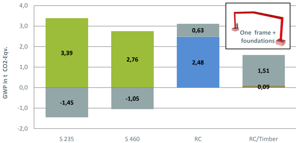
Figure 10: Global Warming Potential for the Product Stage (A1-A3) and separately Benefits & Loads (D, grey) from recycling (steel), incineration (timber) or rubble processing (concrete) for one frame with foundations, in t CO 2 Equivalent
