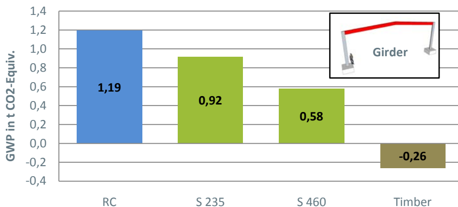
Figure 20: Global Warming Potential for the Product Stage (A1-A3) summed up with Benefits & Loads (D) from recycling (steel), incineration (timber) or rubble processing (concrete) for one girder, in t CO2-Equivalent
