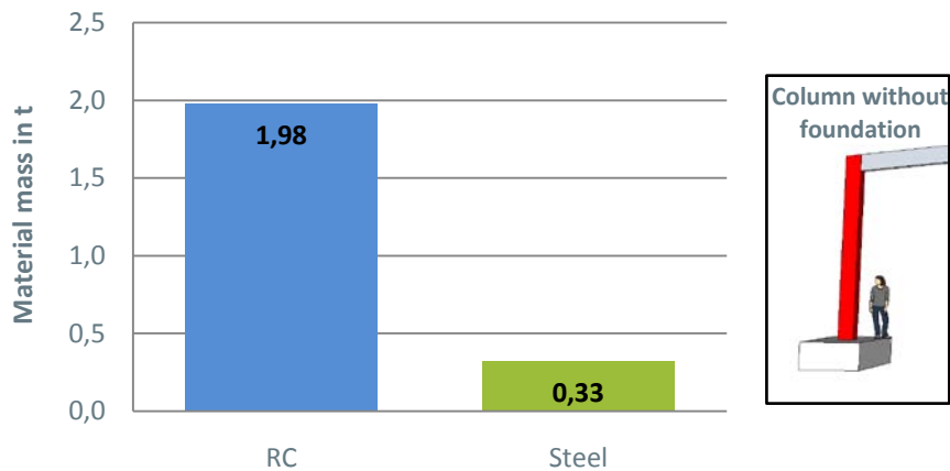
Figure 16: Quantities for columns without foundation, in t
