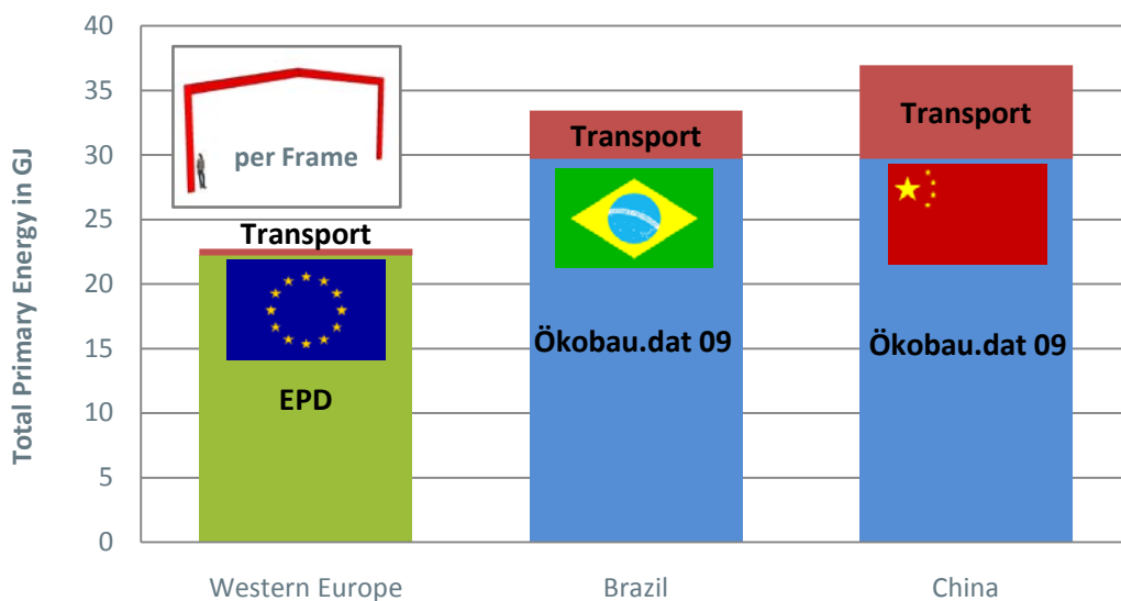
Figure 27: Total Primary Energy for a steel frame S235 including Transport (A4) from gate to site, in GJ
