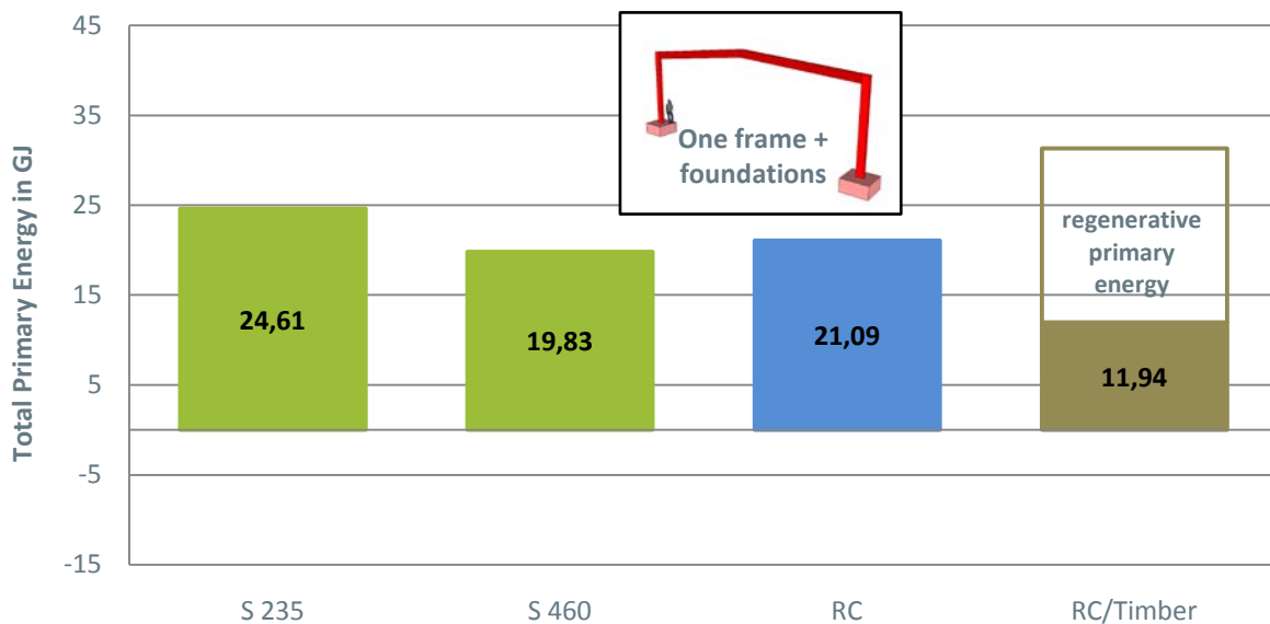
Figure 13: Total Primary Energy for the Product Stage (A1-A3) summed up with Benefits & Loads (D) from recycling (steel), incineration (timber) or rubble processing (concrete) for one frame with foundations, in GJ
