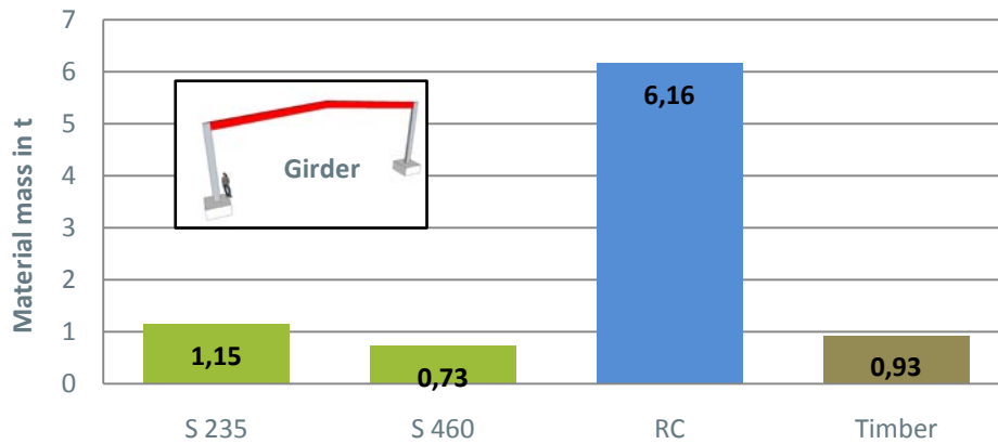
Figure 19: Quantities for a girder, in t
