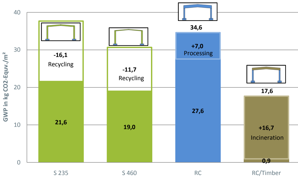
Figure 14: Global Warming Potential for the Product Stage (A1-A3) summed up with Benefits & Loads (D) from recycling (steel), incineration (timber) or rubble processing (concrete) for one frame with foundations, in CO2-Equivalent per m² floor area
